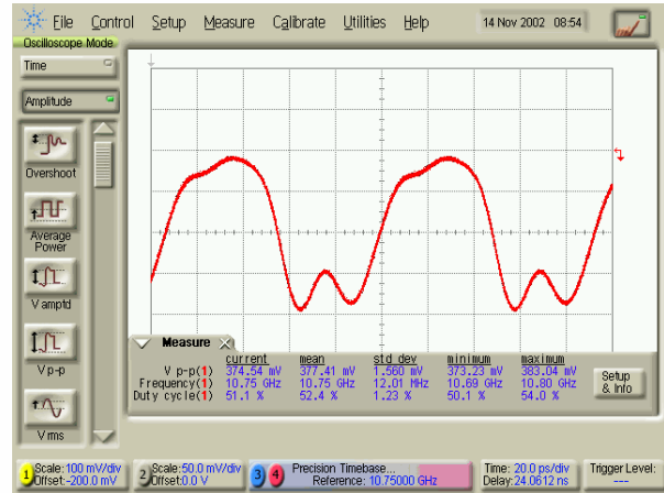
Clock/2 output at 43 Gbps output data rate
