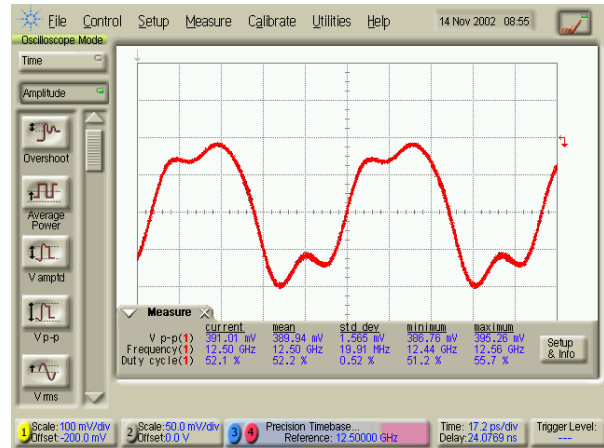
Clock/2 output at 50 Gbps output data rate
