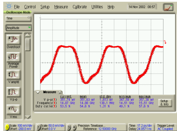
Clock/2 output at 60 Gbps output data rate
