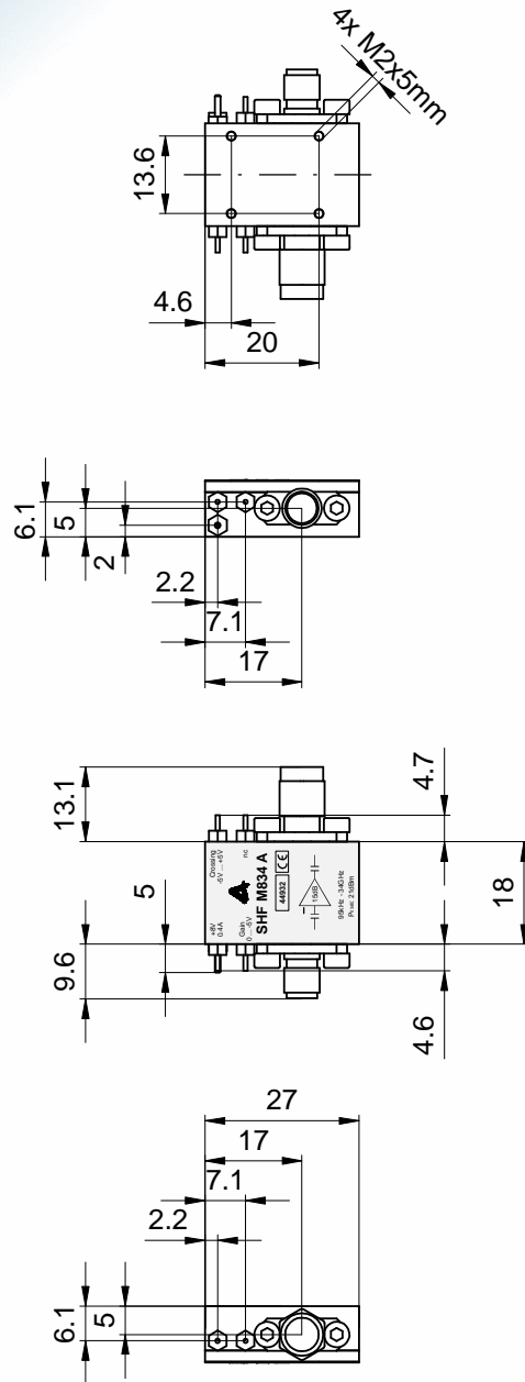
All dimensions in mm
