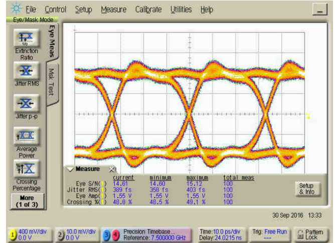
Output Signal @ 30 Gbps, Eye amp: 1.55 V
