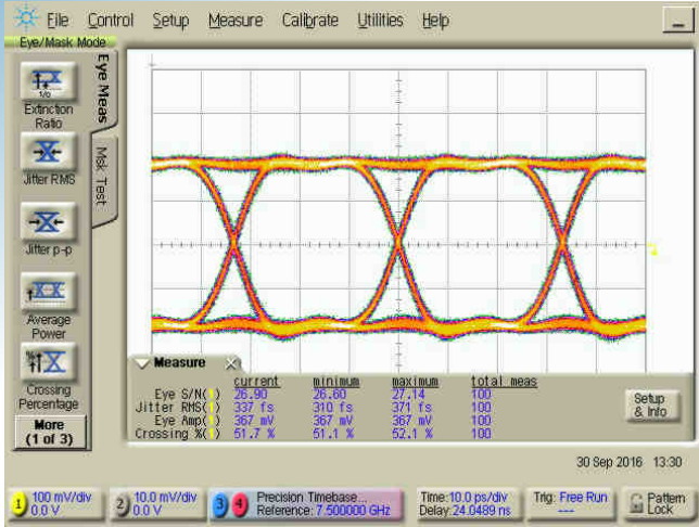
Input Signal @ 30 Gbps, Eye amp: 367 mV
