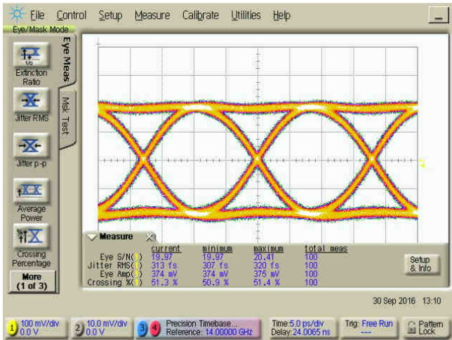
Input Signal @ 56 Gbps, Eye amp: 374 mV
