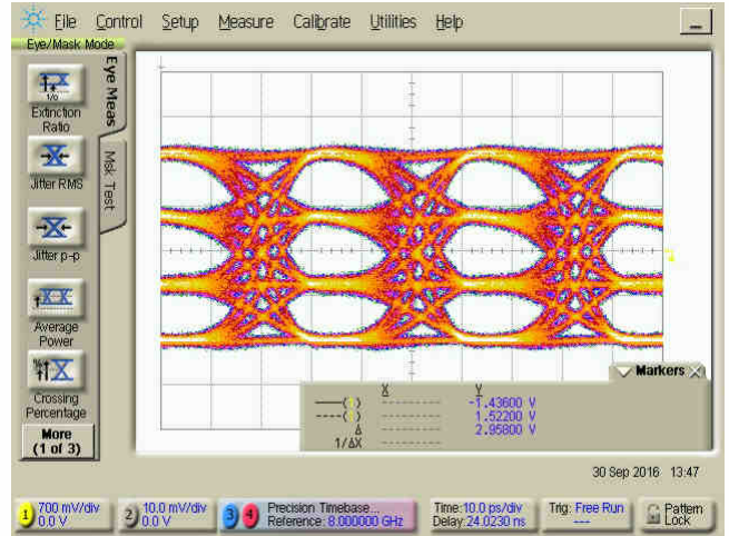
Output Signal @ 32 GBaud, ~3 Vpp
