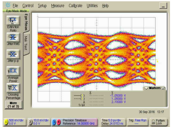
Output Signal @ 56 GBaud, ~2.1 Vpp
