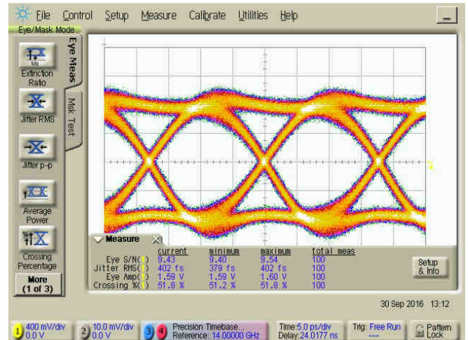
Output Signal @ 56 Gbps, Eye amp: 1.59 V
