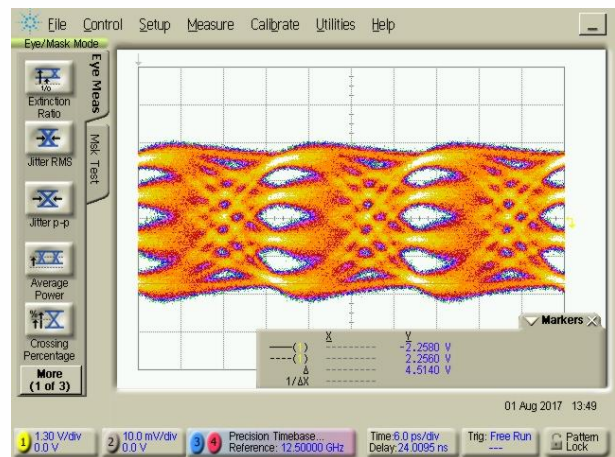
Output Signal @ 50 GBaud, ~4.5 Vpp
