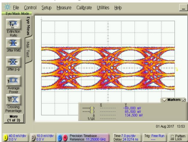
Input Signal @ 45 GBaud
