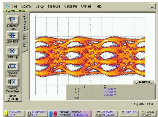
Output Signal @ 45 GBaud, ~4.5 Vpp
