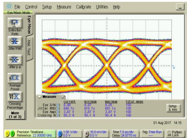
Output Signal @ 44 Gbps
