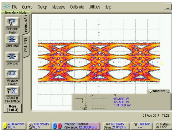
Input Signal @ 50 GBaud
