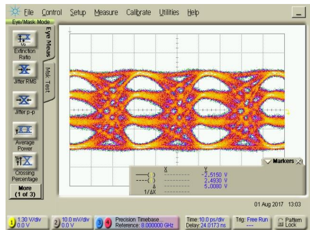
Output Signal @ 32 GBaud, ~5 Vpp
