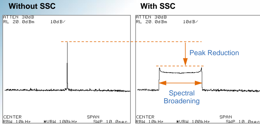
SHF 78120 D clock spectrum with and without SSC.
