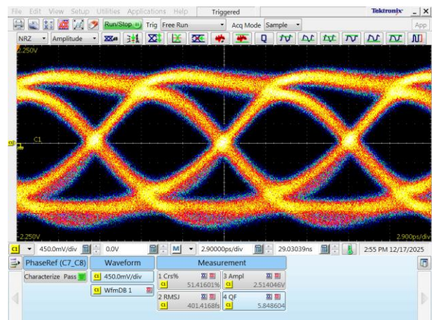
112 Gbps 2.5 V Output Signal
