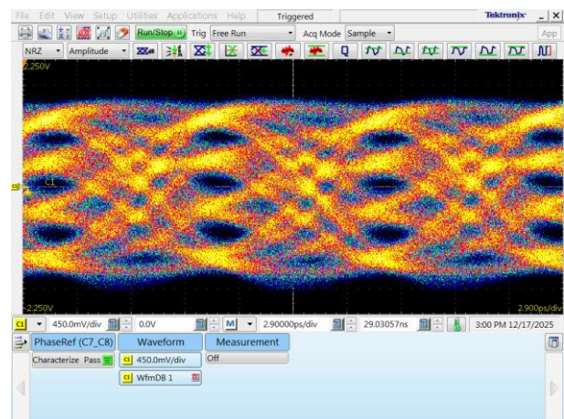
112 GBaud (224 Gbps) 2.5 V Output Signal
