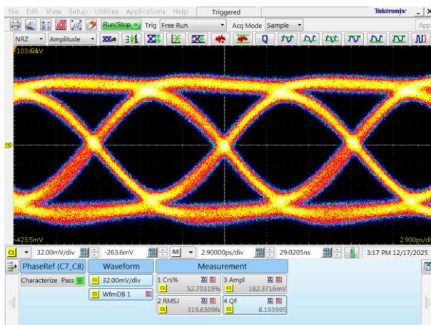
112 Gbps 180 mV Input Signal
