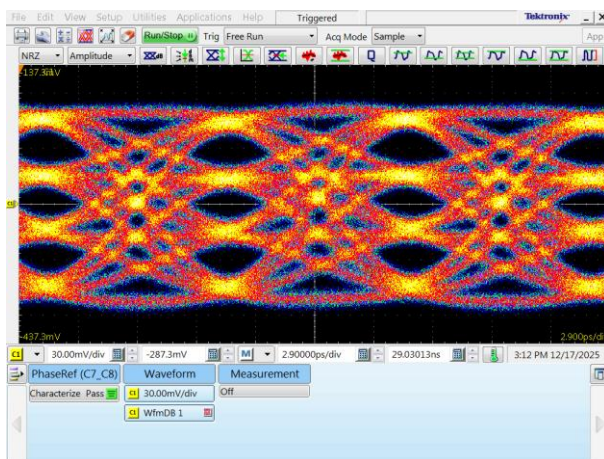
112 GBaud (224 Gbps) 180 mV Input Signal
