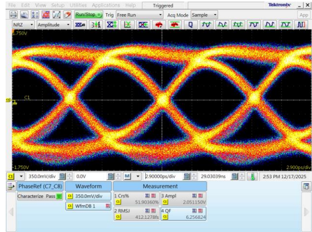
112 Gbps 2.0 V Output Signal
