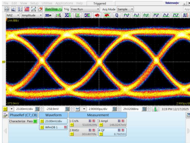
112 Gbps 145 mV Input Signal
