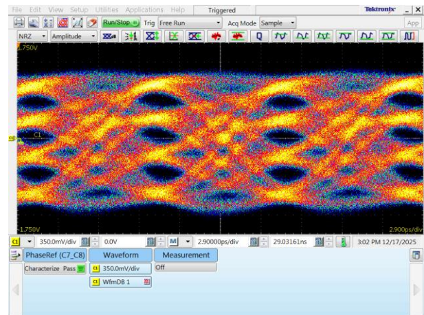
112 GBaud (224 Gbps) 2.0 V Output Signal
